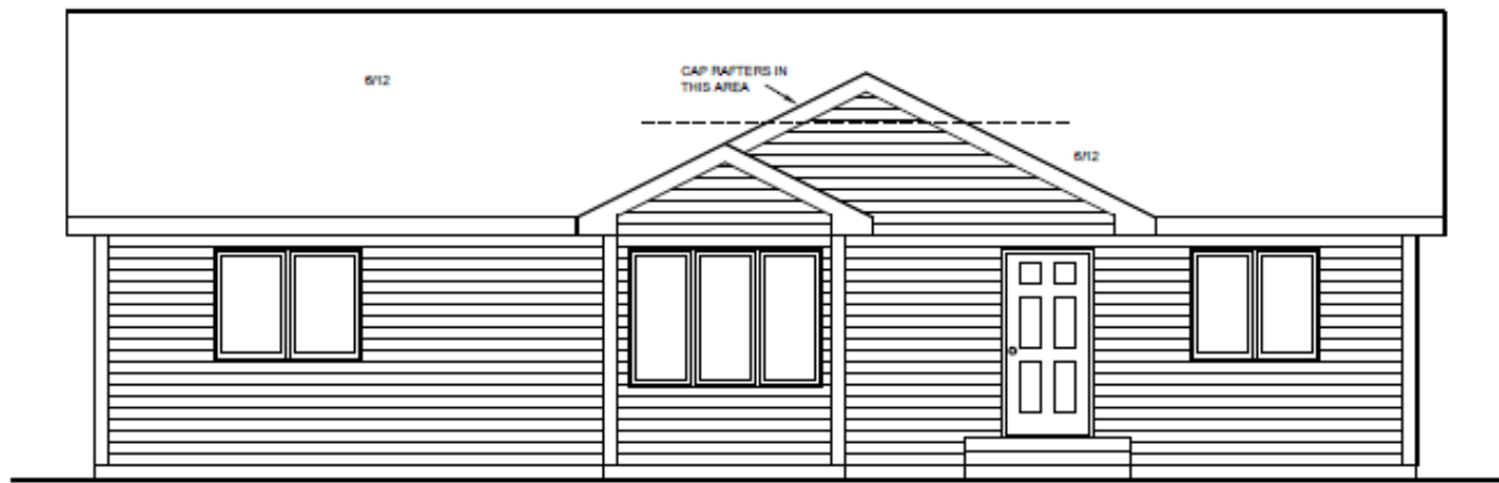
FRONT ELEVATION 1/4" = 1'-0"
