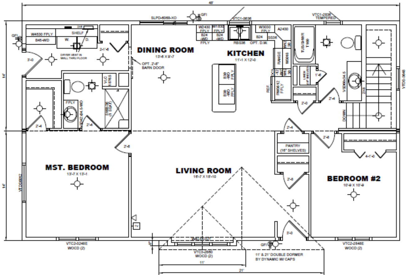
FLOOR PLAN 1/4" = 1'-0" (DIMENSIONS FRAMING TO FRAMING)
