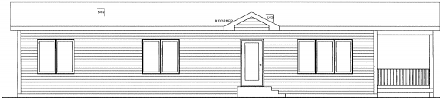
FRONT ELEVATION 1/4"=1'-0" (DIMENSIONS FRAMING TO FRAMING)
