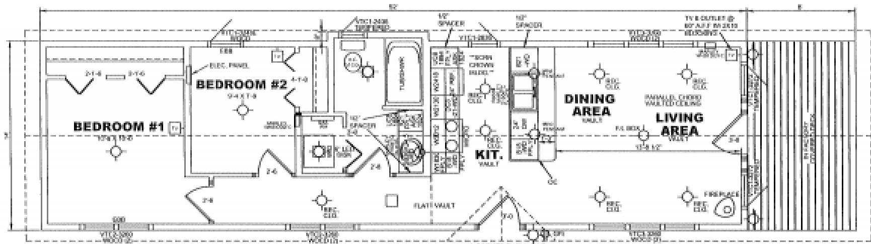
FLOOR PLAN 728 SQ. FT. LIVING AREA 1/4"=1'-0" (DIMENSIONS FRAMING TO FRAMING)
